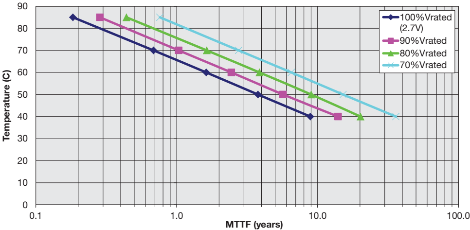
Expected Lifetime at Various Voltages SCC series 2.7V Rated
