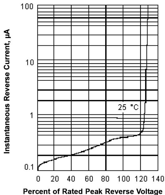
Fig. 1-Typical Reverse Characteristics
