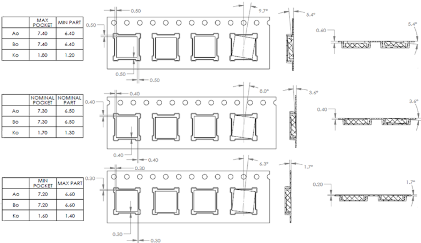
Figure 9.3. Tape information
