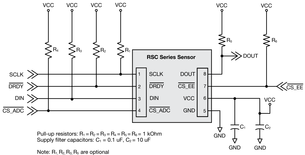
Figure 6. Recommended Circuit
