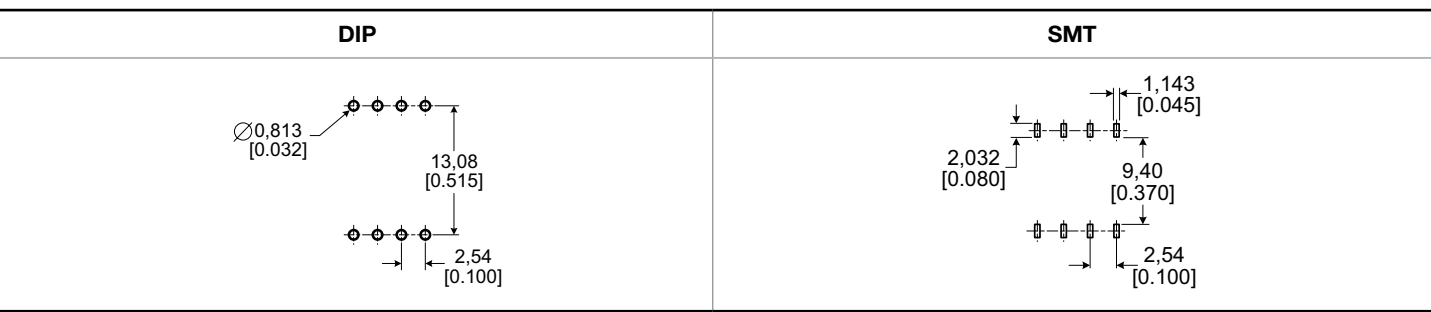
Figure 5. Recommended PCB Pad Layouts
