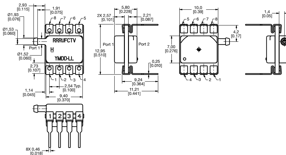
Figure 3. DIP Package Dimensional Drawings (continued)
