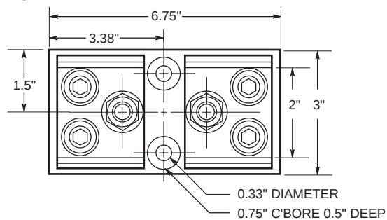
Figure 6. 401A to 600A
