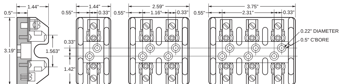
Figure 1. ½A to 30A All dimensions (± 0.016)
