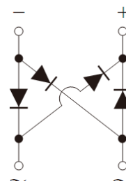
TO-269AA (MBS)
