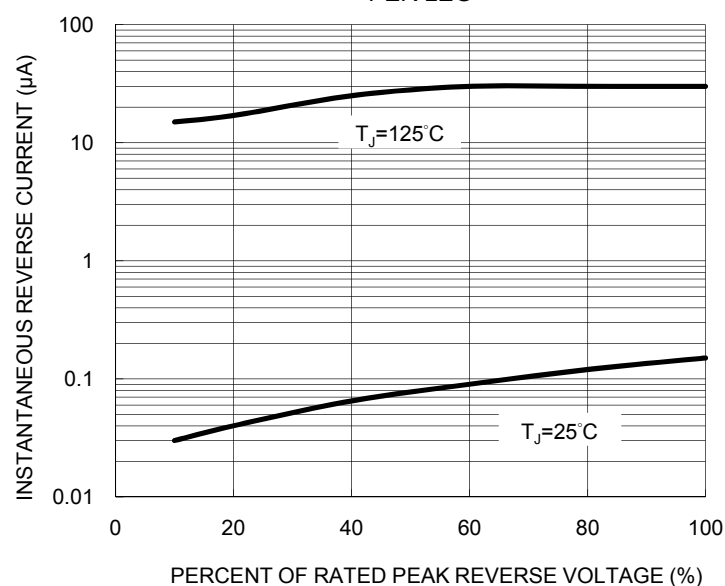
FIG. 2 TYPICAL REVERSE CHARACTERISTICS PER LEG
