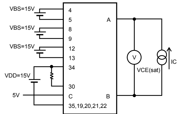
Figure 26. Test circuit for V_{CE(sat)}
