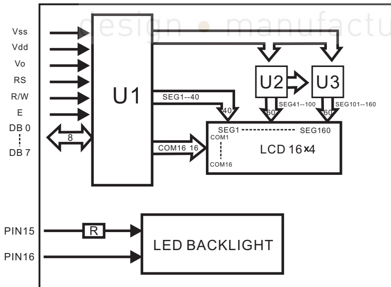
Block Diagram
