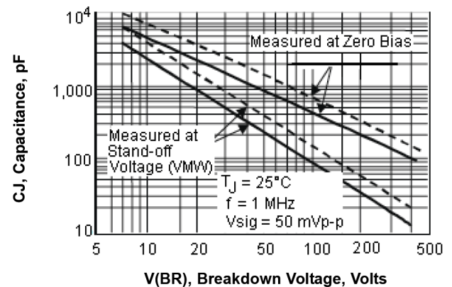
Fig. 4-Typical Junction Capacitance Unidirectional
