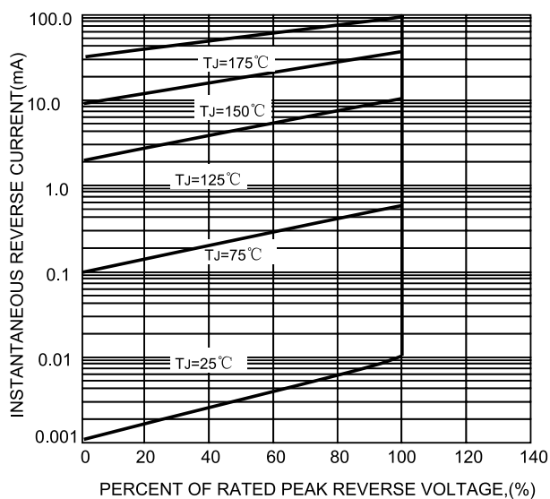
FIG.3-TYPICAL REVER CHARACTERISTICS
