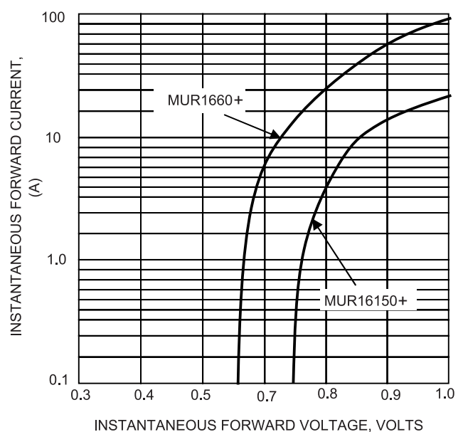
FIG.4-TYPICAL FORWARD CHARACTERISTICS
