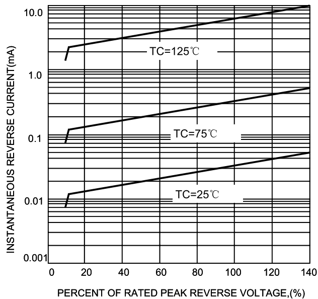
FIG.3-TYPICAL REVER CHARACTERISTICS
