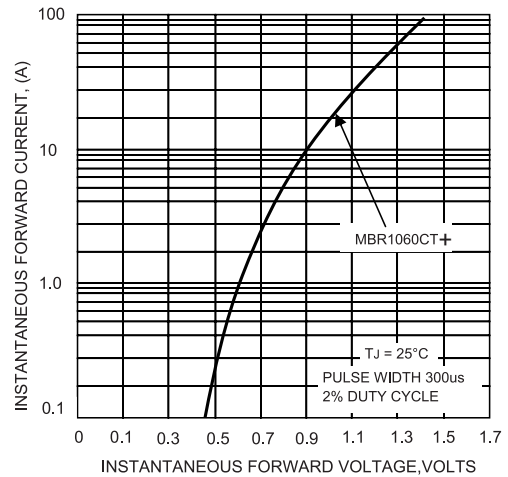
FIG.4-TYPICAL FORWARD CHARACTERISTICS
