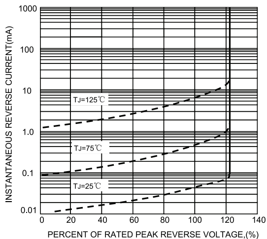
FIG.3-TYPICAL REVERSE
