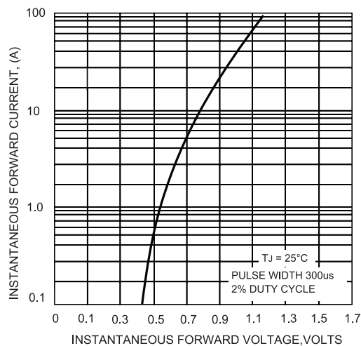
FIG.4-TYPICAL FORWARD CHARACTERISTICS
