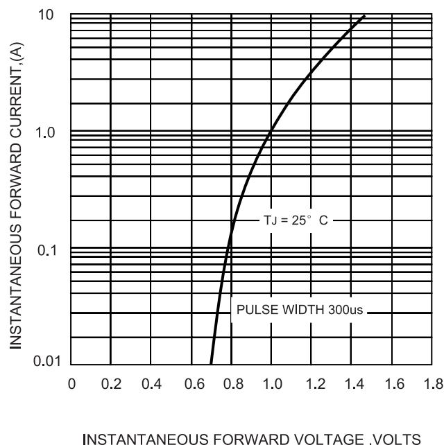
FIG.4-TYPICAL FORWARD CHARACTERISTICS
