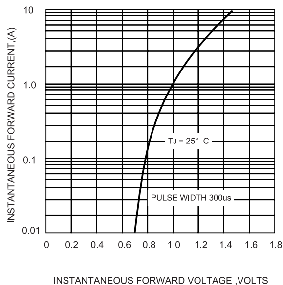
FIG.4-TYPICAL FORWARD CHARACTERISTICS
