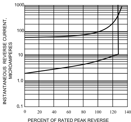
FIG.5-TYPICAL REVERSE CHARACTERISTICS
