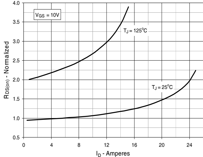
Fig. 5. R_{DS(on)} Normalized to I_D = 6A Value vs. Drain Current
