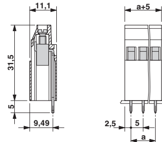
Dimensional drawing
