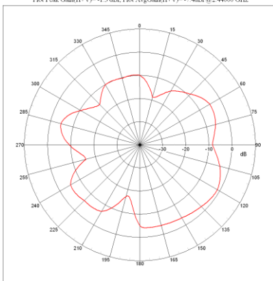
Far-field Power Distribution(H+V) on X-Z Plane Plot Peak Gain(H+V)=-1.3 dBi, Plot AvgGain(H+V)=-7.4dBi @2.44000 GHz
