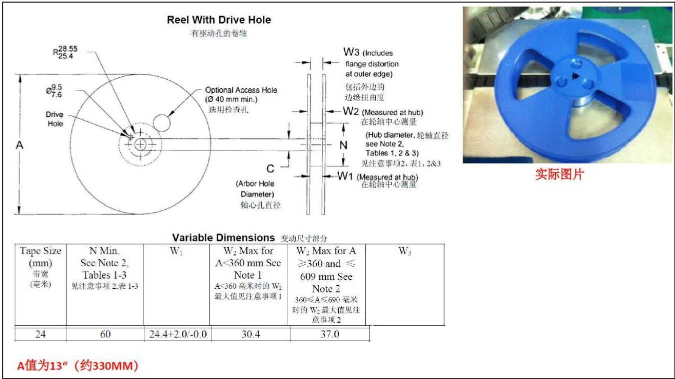
Figure 12: Reel specifications
