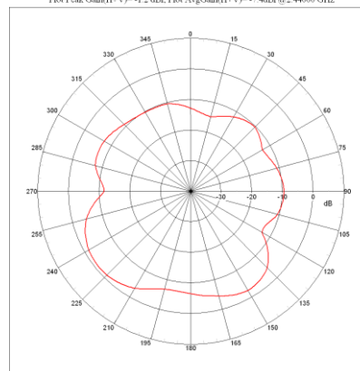
Far-field Power Distribution(H+V) on Y-Z Plane Plot Peak Gain(H+V)=-1.2 dBi, Plot AvgGain(H+V)=-7.4dBi @2.44000 GHz
