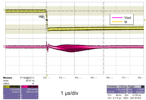
Figure 14: dv/dt
