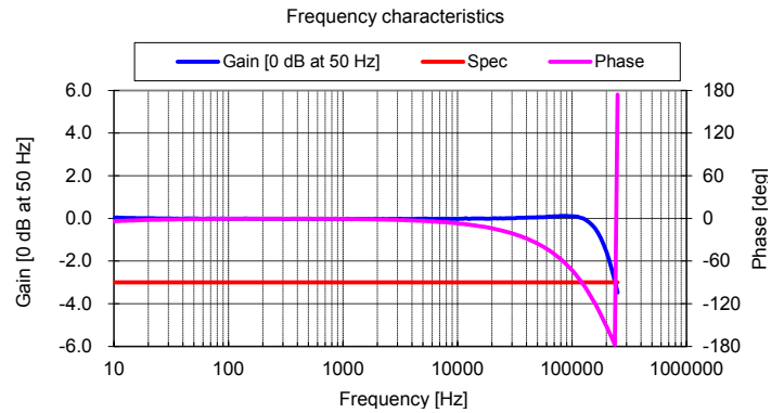
Figure 2: Frequency response
