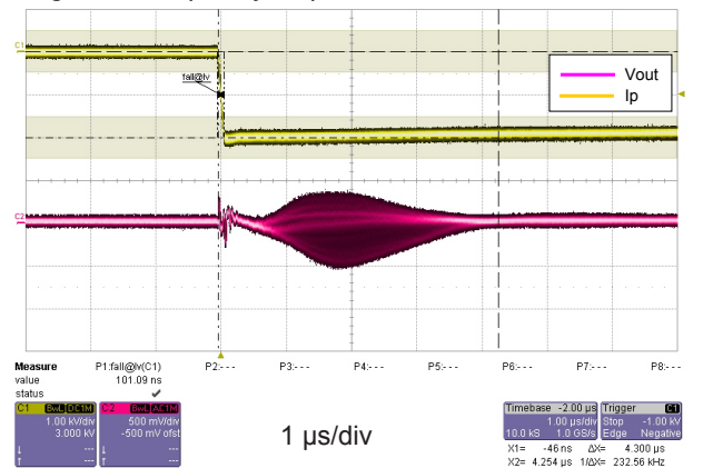
Figure 4: dv/dt
