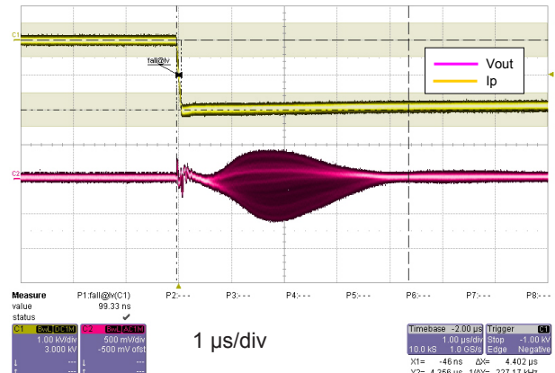
Figure 9: dv/dt
