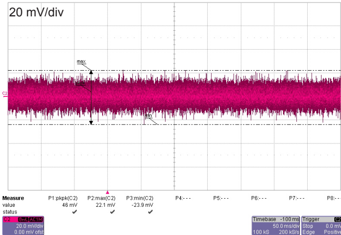
Figure 10: Output noise
