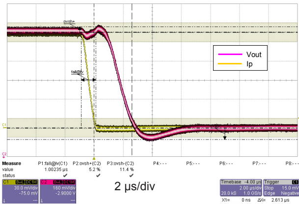
Figure 8: Step response
