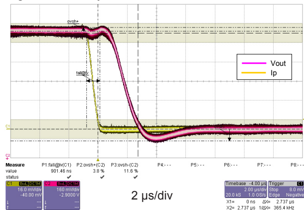
Figure 3: Step response
