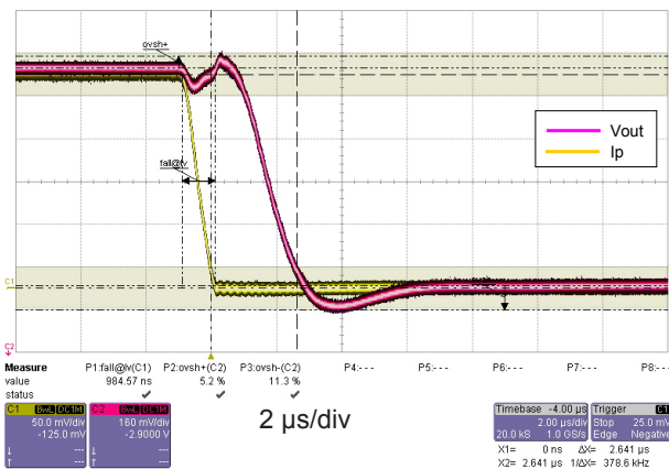
Figure 13: Step response
