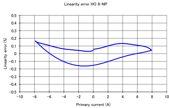
Figure 1: Linearity error
