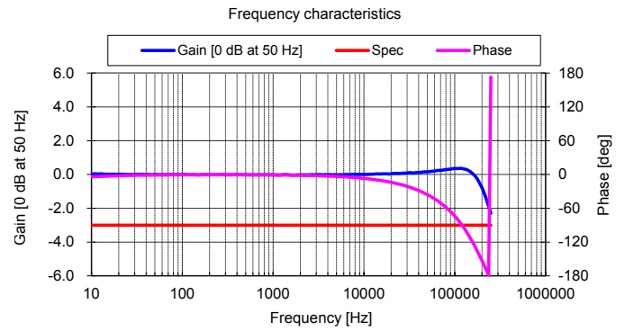
Figure 12: Frequency response
