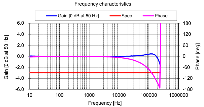
Figure 7: Frequency response
