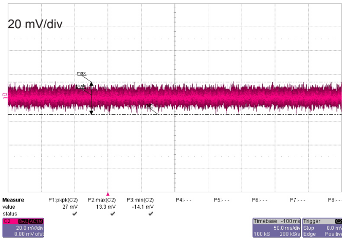
Figure 15: Output noise
