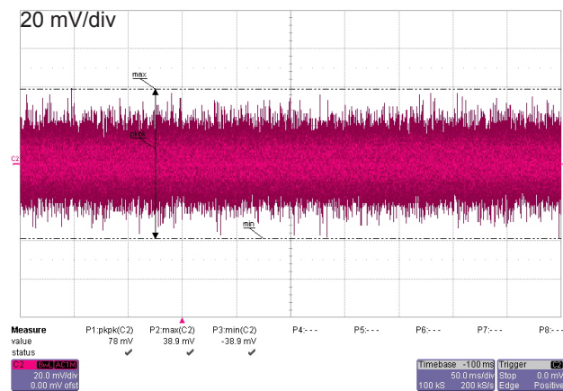
Figure 5: Output noise
