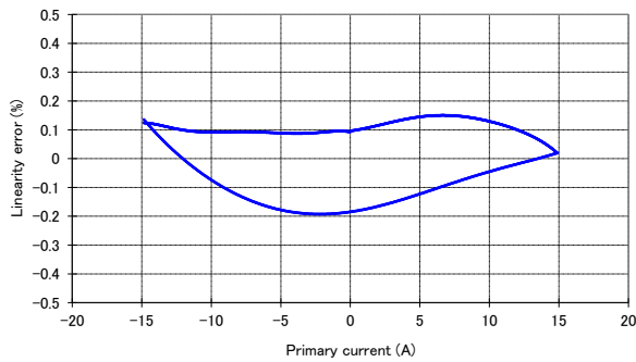
Figure 6: Linearity error
