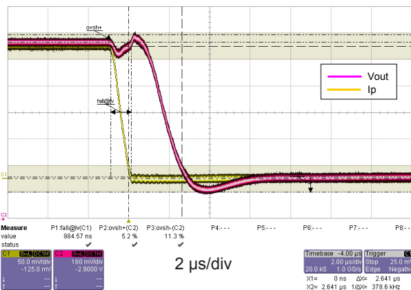
Figure 13: Step response
