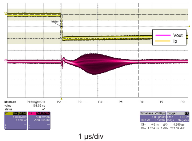
Figure 4: dv/dt
