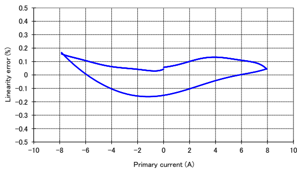
Figure 1: Linearity error
