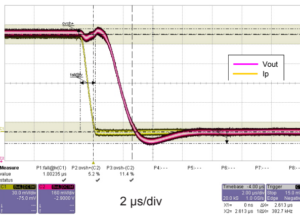
Figure 8: Step response
