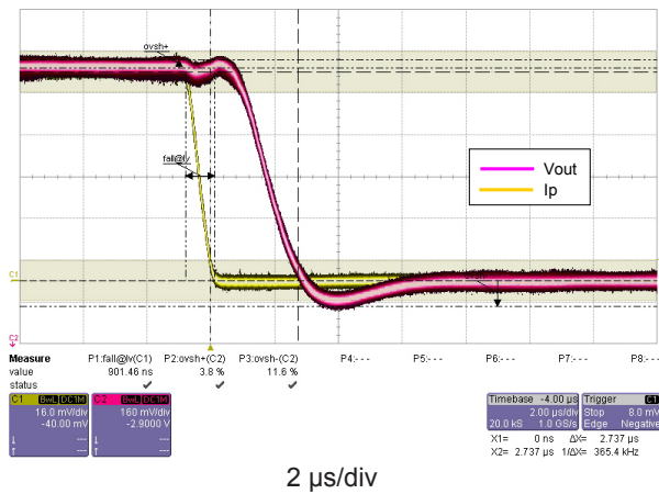
Figure 3: Step response
