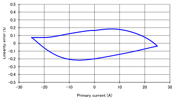
Figure 11: Linearity error
