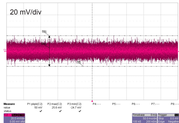
Figure 10: Output noise
