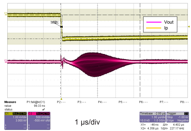
Figure 9: dv/dt
