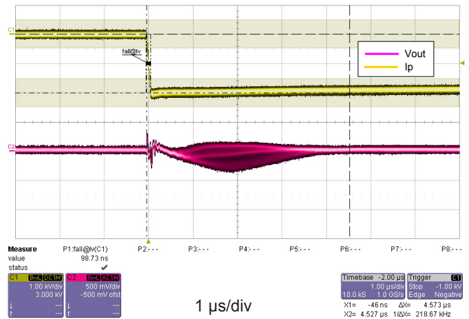
Figure 14: dv/dt
