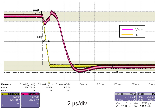
Figure 13: Step response
