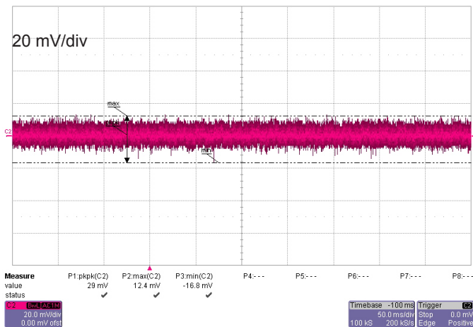
Figure 10: Output noise
