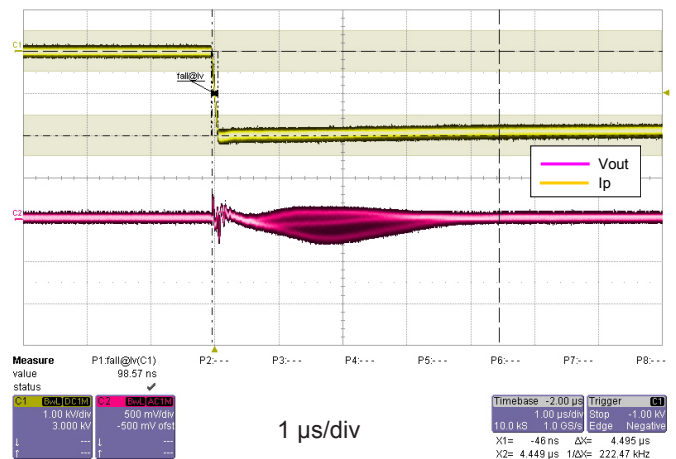
Figure 9: dv/dt
