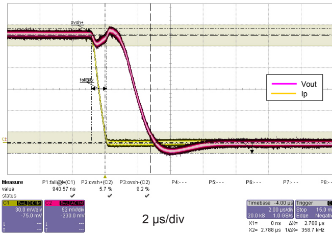
Figure 8: Step response
