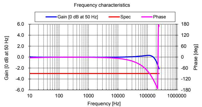
Figure 7: Frequency response
