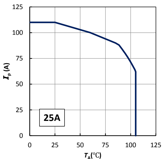
Figure 16: I_p vs T_A for HO series
