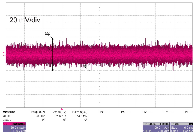
Figure 5: Output noise
