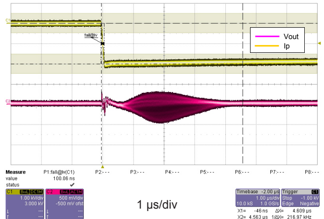
Figure 4: dv/dt
