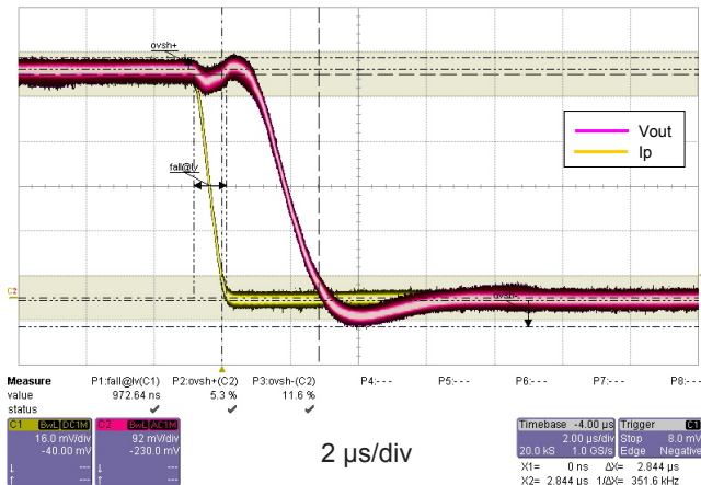
Figure 3: Step response
