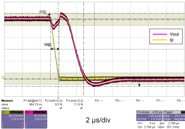
Figure 13: Step response
