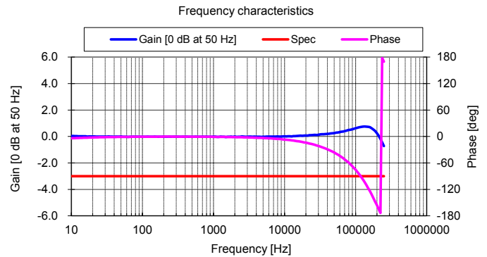
Figure 12: Frequency response
