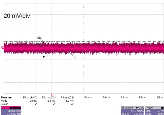
Figure 10: Output noise
