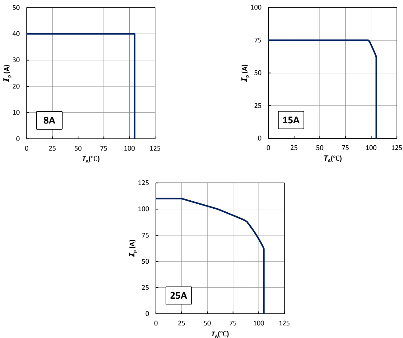
Figure 16: I_p vs T_A for HO series
