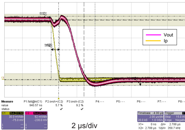
Figure 8: Step response
