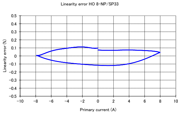
Figure 1: Linearity error
