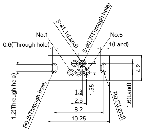
PCB mounting pattern
