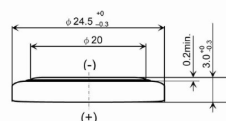
Dimension Drawing
