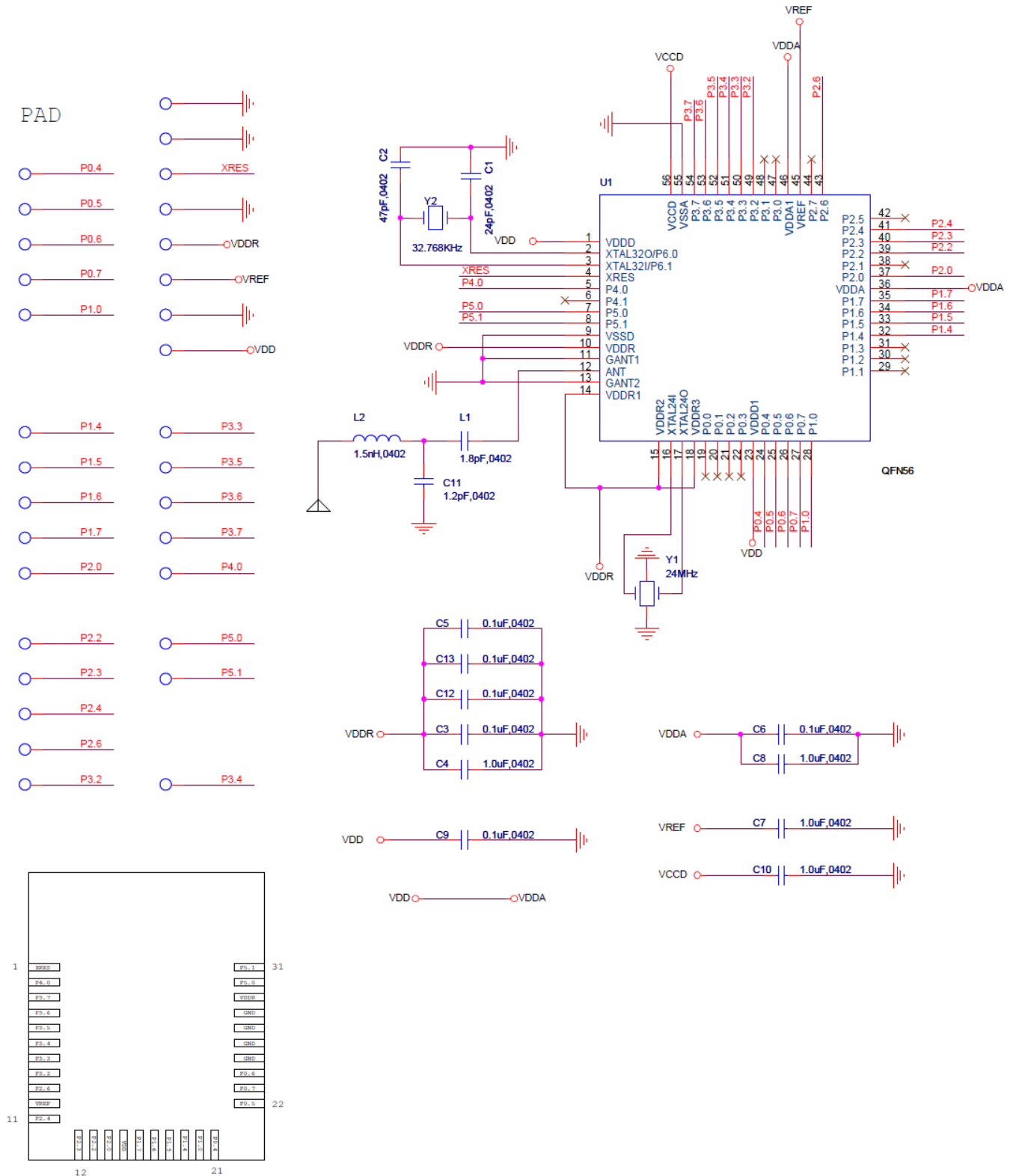
Figure 9. CYBLE-01201X-X0 Schematic Diagram
