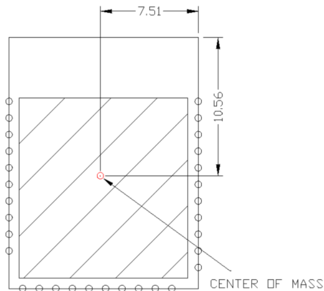
Figure 13. CYBLE-01201X-X0 Center of Mass (Seen from Top)
