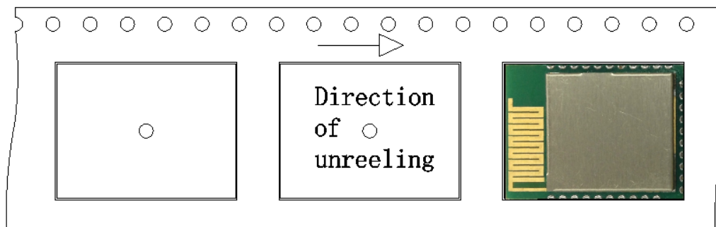
Figure 11. Component Orientation in Tape and Unreeling Direction
