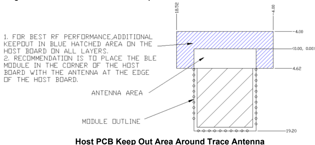
Figure 3. Recommended Host PCB Keep Out Area Around the CYBLE-01201X-X0 Antenna
