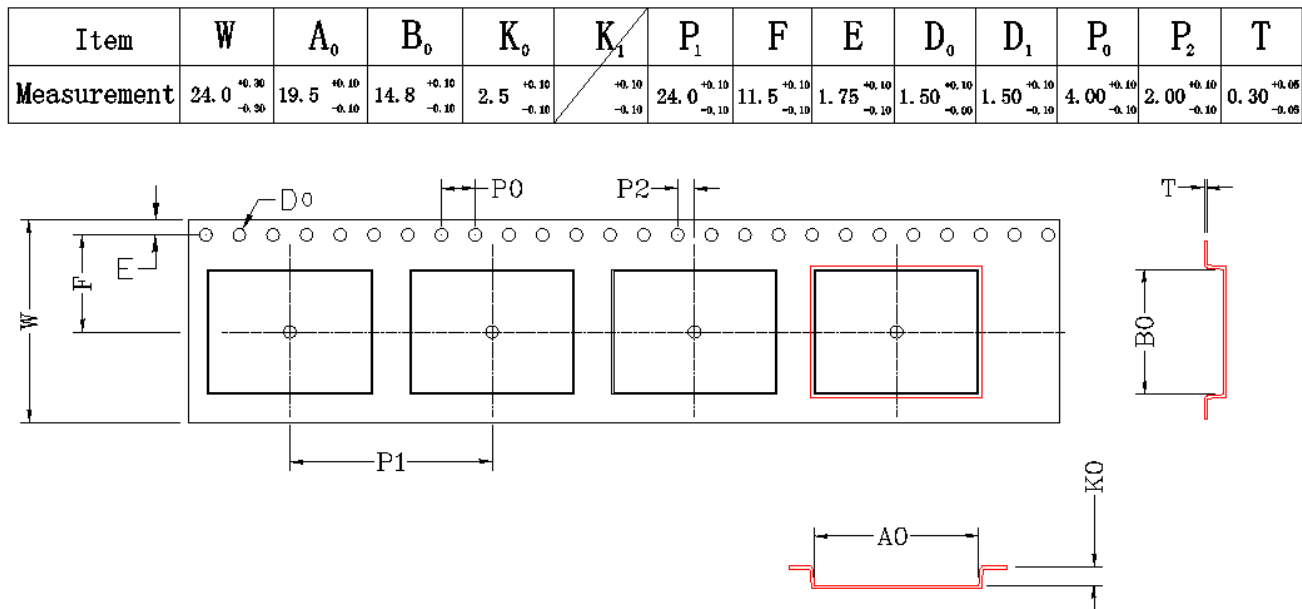
Figure 10. CYBLE-01201X-X0 Tape Dimensions
