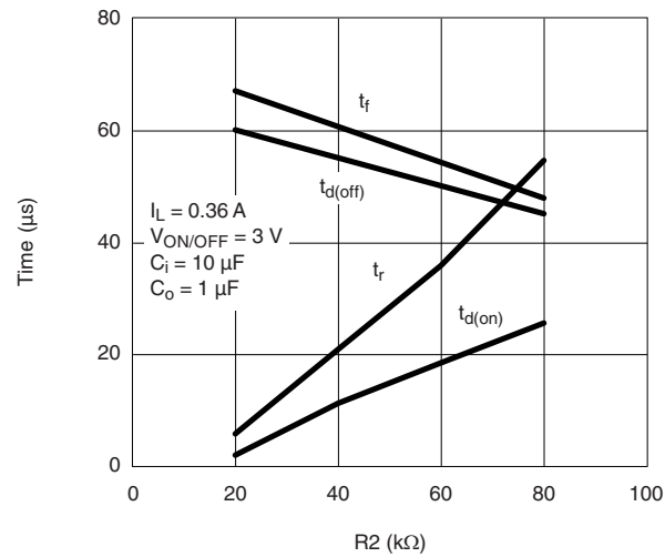
Switching Variation R2 at V_{IN} = 1.8 \text{ V} , R1 = 300 \text{ kΩ}
