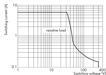
DC load limit curve
