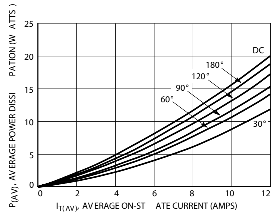
Figure 6. On-State Power Dissipation
