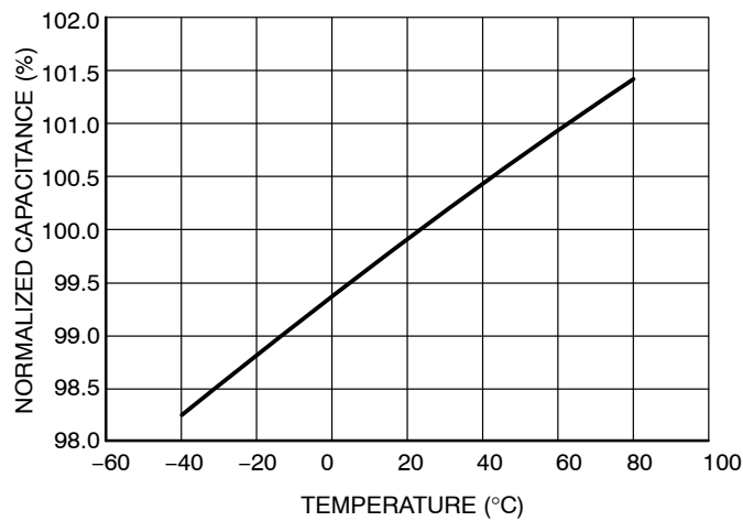
Figure 8. Normalized Capacitance over Temperature (Normalized @ 25°C, V R = 2.5 V, f = 1 MHz)
