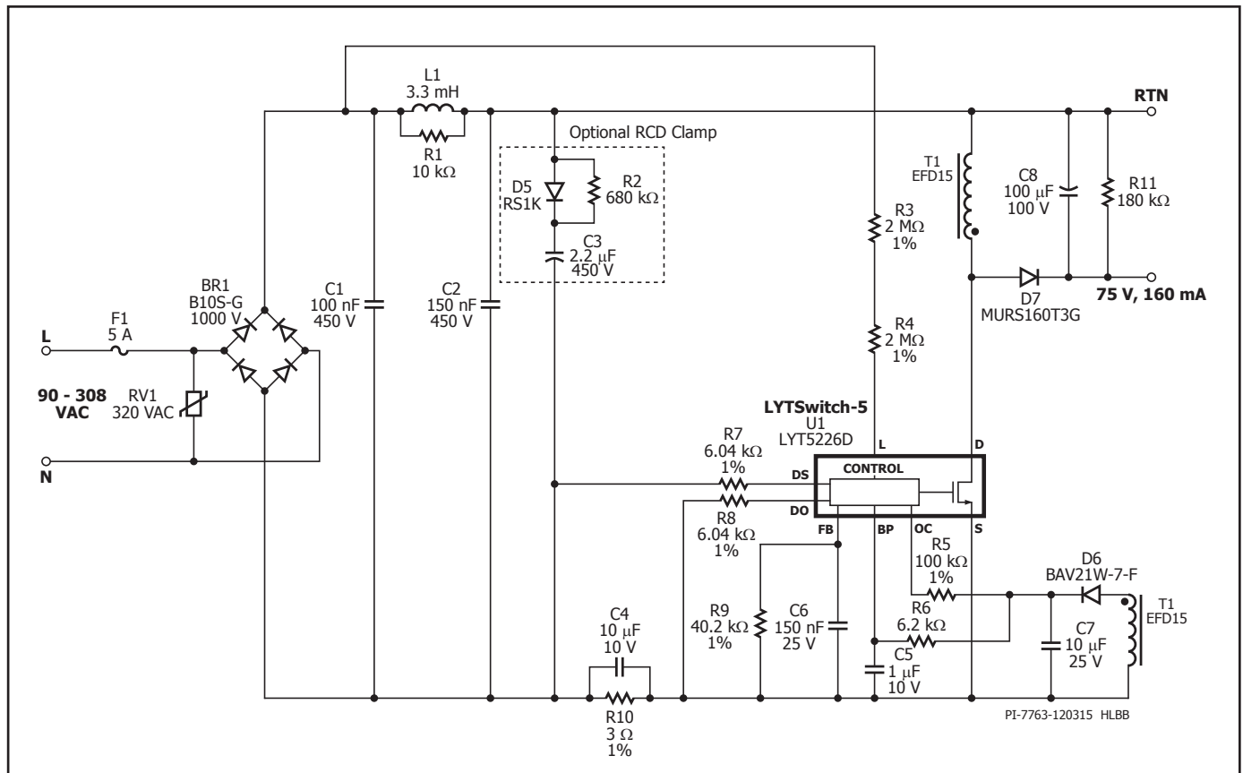
Figure 5. 12 W, 75 V, 160 mA Non-Isolated Tube Lamp Driver for Wide Input Range of 90 VAC to 308 VAC using LYT5226D.
