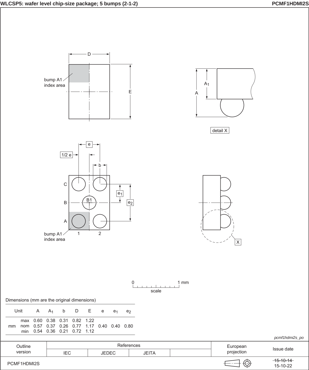
Fig 19. Package outline WLCSP5
