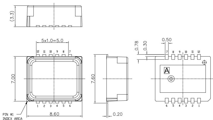
Figure 3. Housing dimensions
