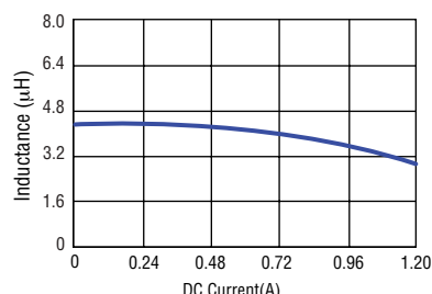
SRN3012TA-4R7M
