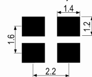
Solder Pad Layout
