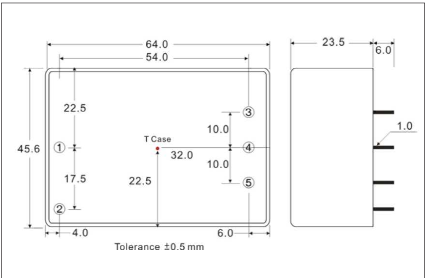
Outline Drawing KMSA30
