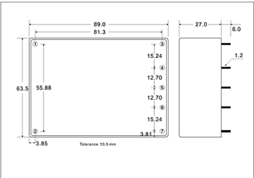
Outline Drawing KMSA60
