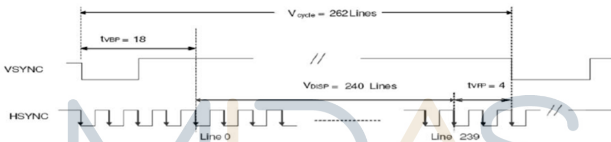
b ) Vertical Data Transaction Timing
