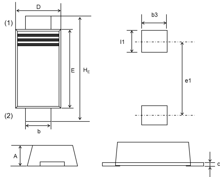
SOD-123FL, (FMDU)
