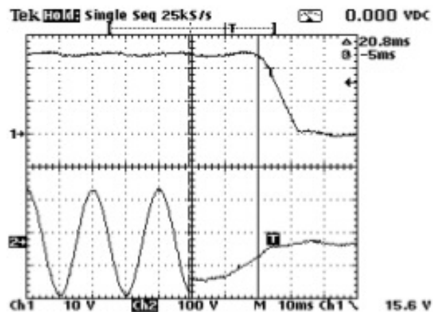
ECM100US24 hold up 115 VAC at 100% load Hold up time is 20.8 ms
