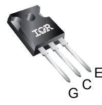
IRGP4790-EPbF TO-247AD
