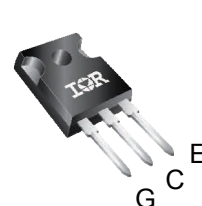
IRGP4790PbF TO-247AC
