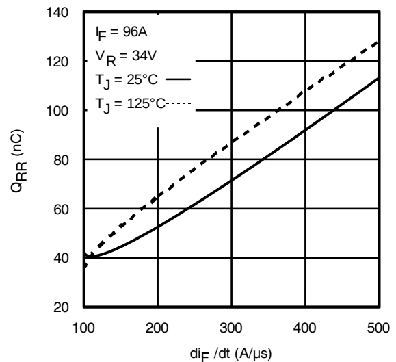
Fig. 19 - Typical Stored Charge vs. d i_F / d t
