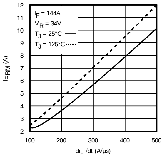
Fig. 18 - Typical Recovery Current vs. d i_F / d t
