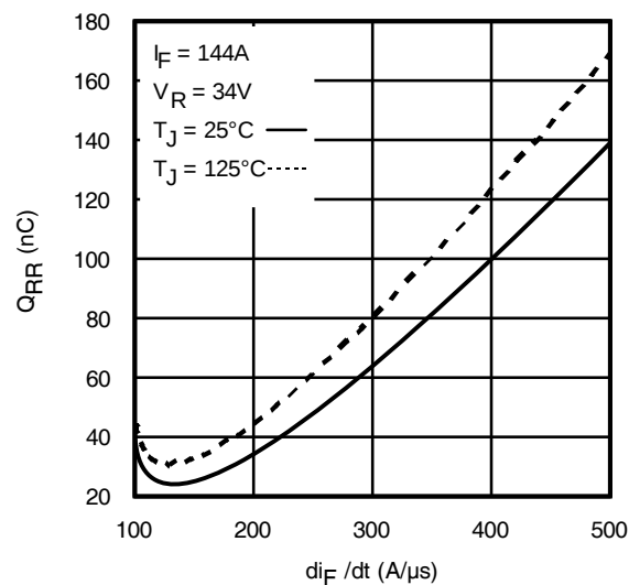
Fig. 20 - Typical Stored Charge vs. d i_F / d t
