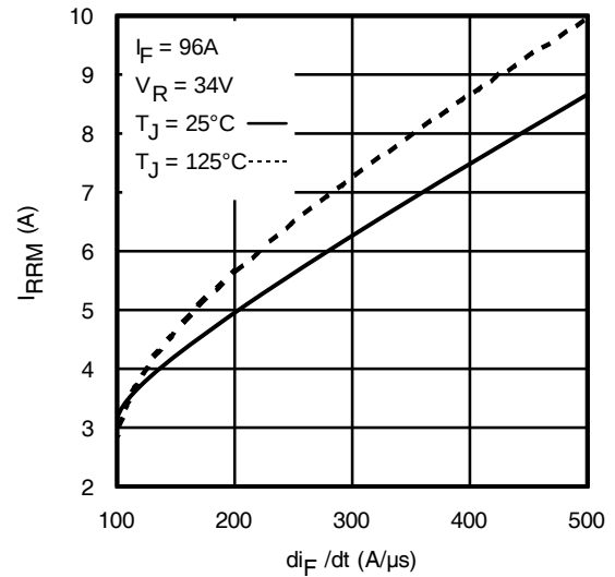
Fig. 17 - Typical Recovery Current vs. d i_F / d t
