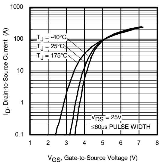
Fig 5. Transfer Characteristics
