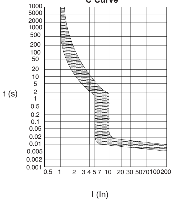
C Curve
