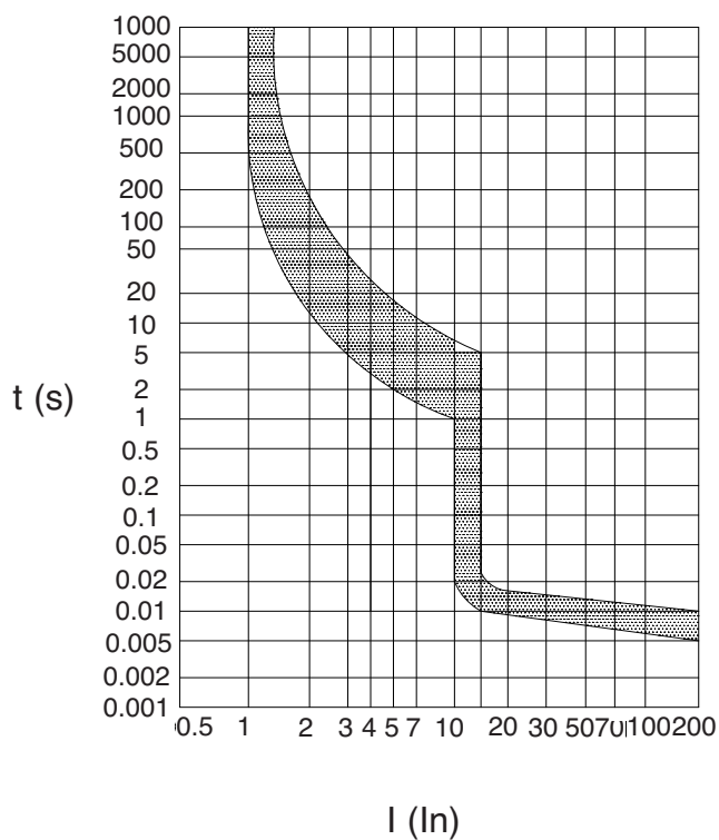
D Curve
