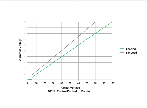
Typical Output vs. Input Voltage
