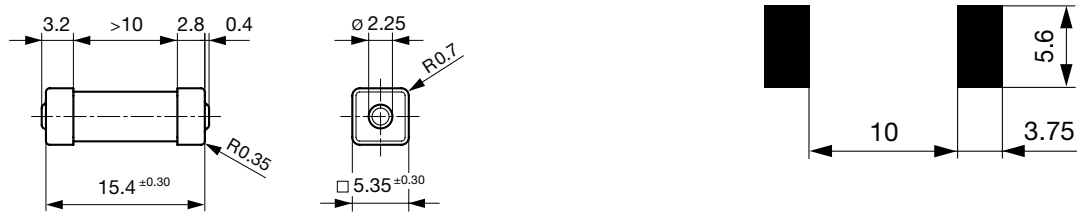
Soldering pads
