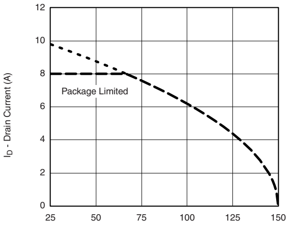
Current Derating*
