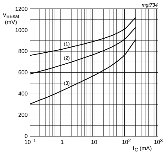
Fig 14. BC847CQA: Base-emitter voltage as a function of collector current; typical values
