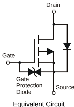
Equivalent Circuit
