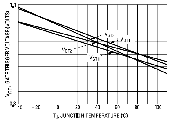
Figure 16. Gate Trigger Voltage Variation
