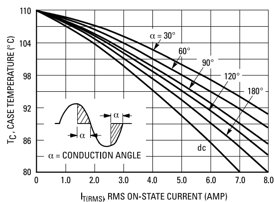
Figure 1. Current Derating
